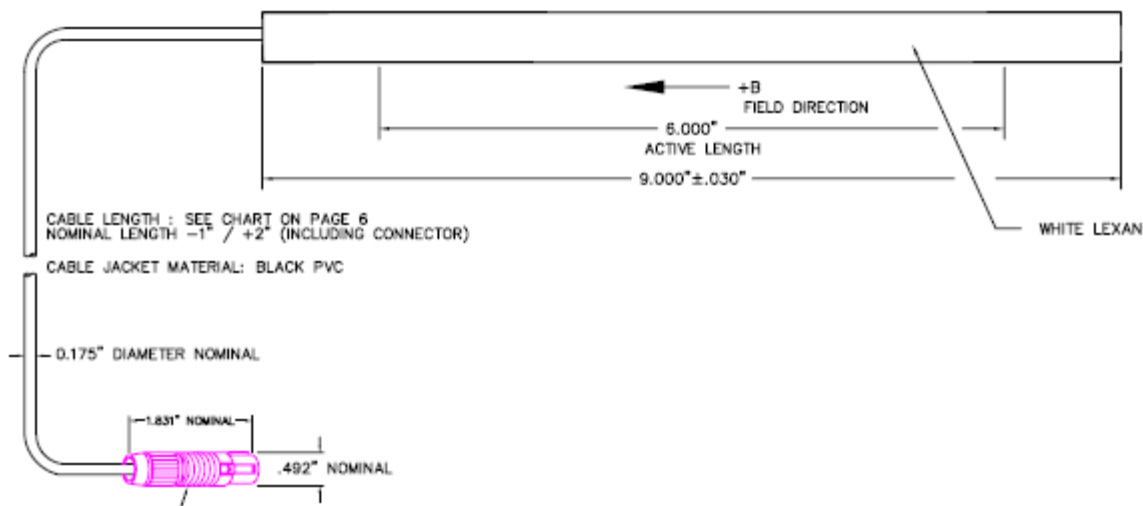
FIGURE 4. MOX Magna Probe
